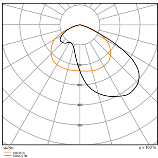
URBAN VLA RET P 60W 730 A60X120
