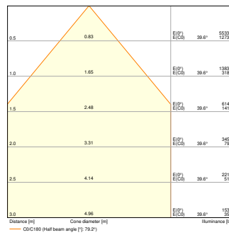
HB DA P 150W 865 110DEG IP66 WITH REFLECTOR
