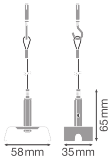
TRUSYS FLEX SUSPENSION KIT
