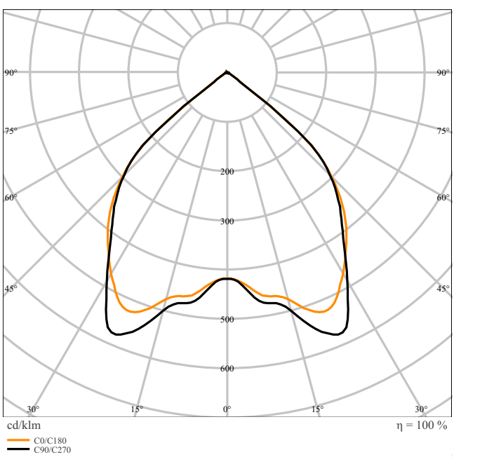
LISOEV 1074X29 46 40W 930 S90U19 BK LEDV 800mA
