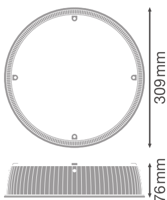
HB PC REFRACTOR 93W
