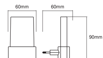
Produkt Line Drawing LUNETTA Shine WT
