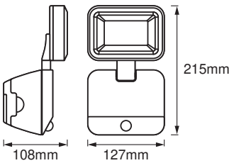
BATTERY LED SPOTLIGHT SINGLE WT OSRAM
