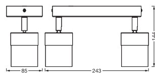
LED SPOT HALF WOOD LINE 2XGU10 WT
