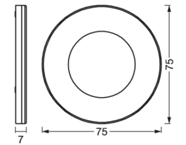
UNDERCABINET SPOTMAGNET
